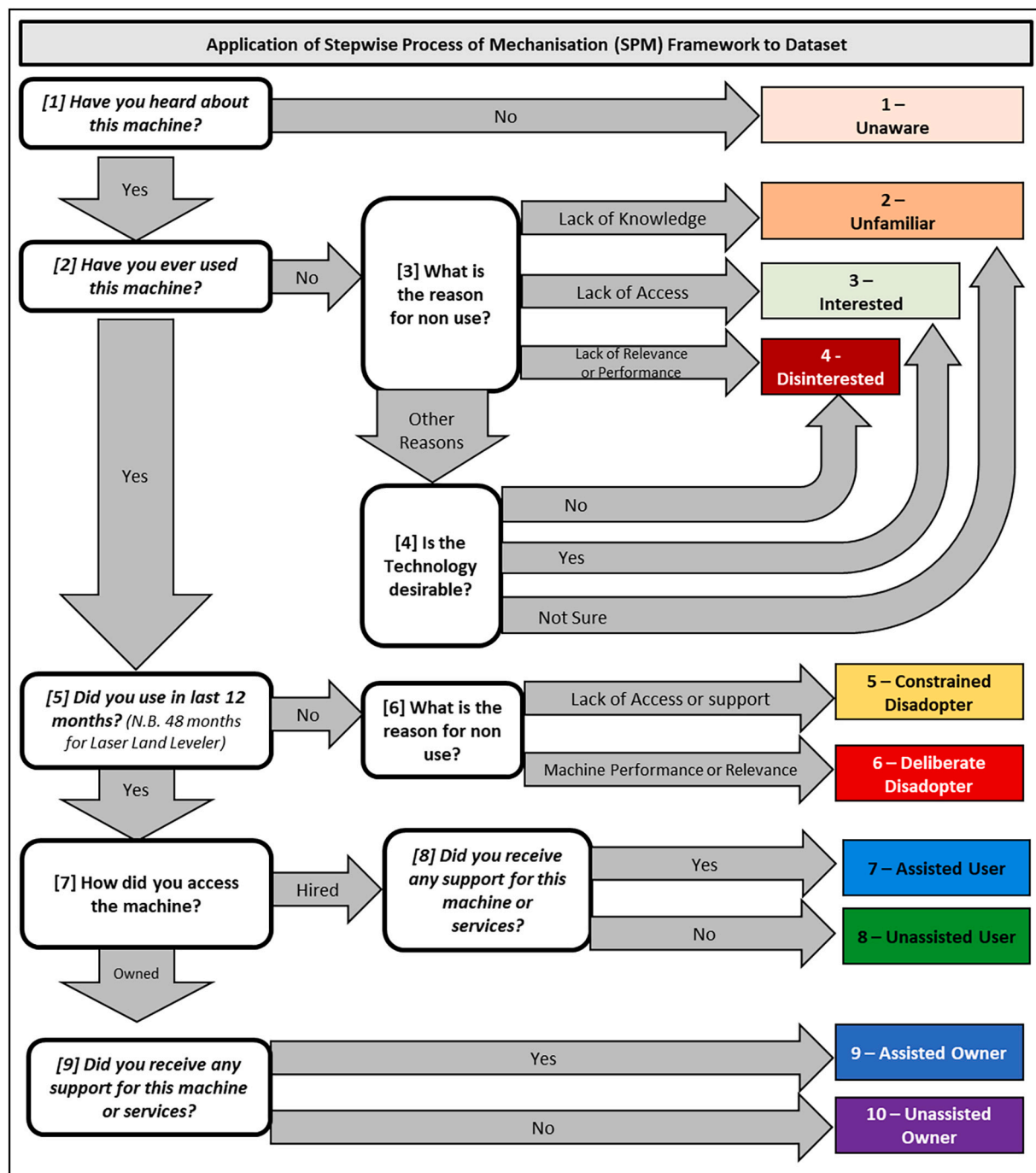
Fig. 4. Analytical framework for implementation of the SPM Framework. Note the theoretical framework is dynamic with feedback loops (noted with grey arrows), while the analytical framework is static to capture a point in time.
